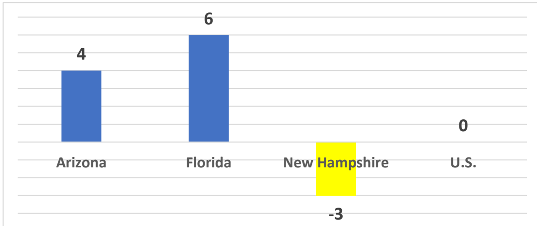
Figure 16. Change in NAEP Grade 8 Reading Scores, 2003 to 2019
